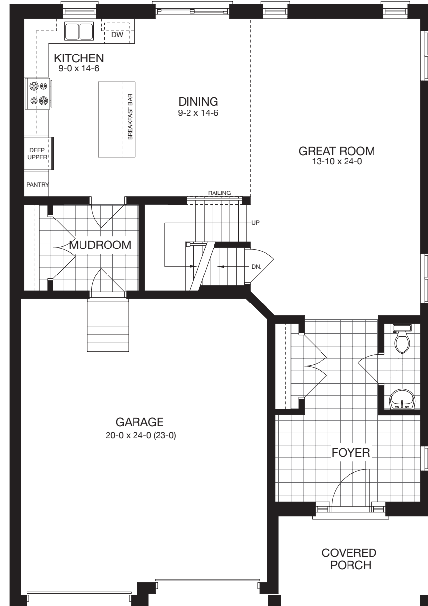
Main Floor
