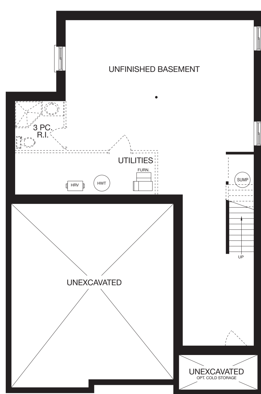
Basement
