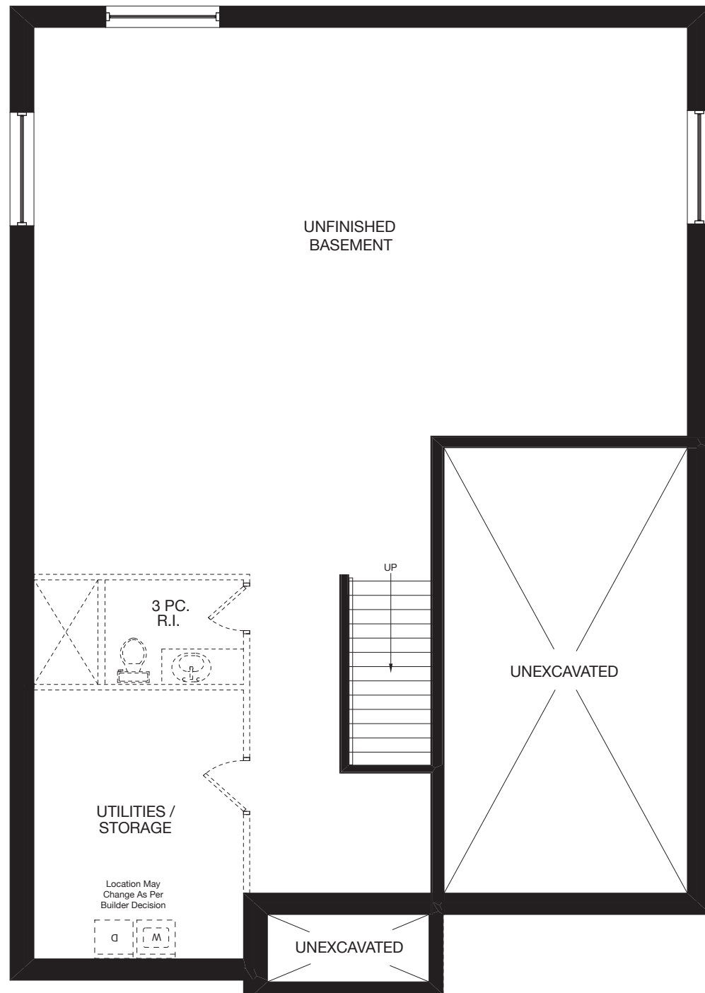
BASEMENT
