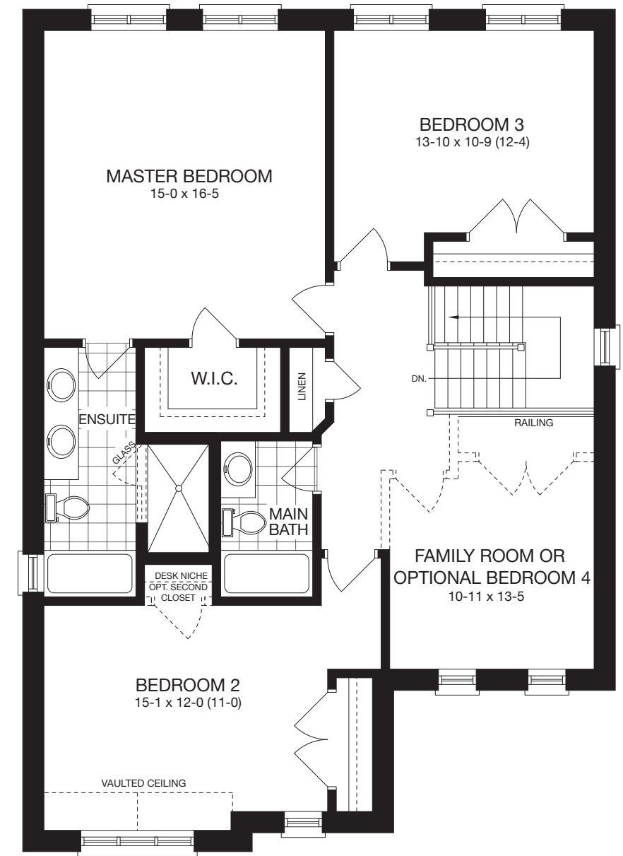
Second Floor
