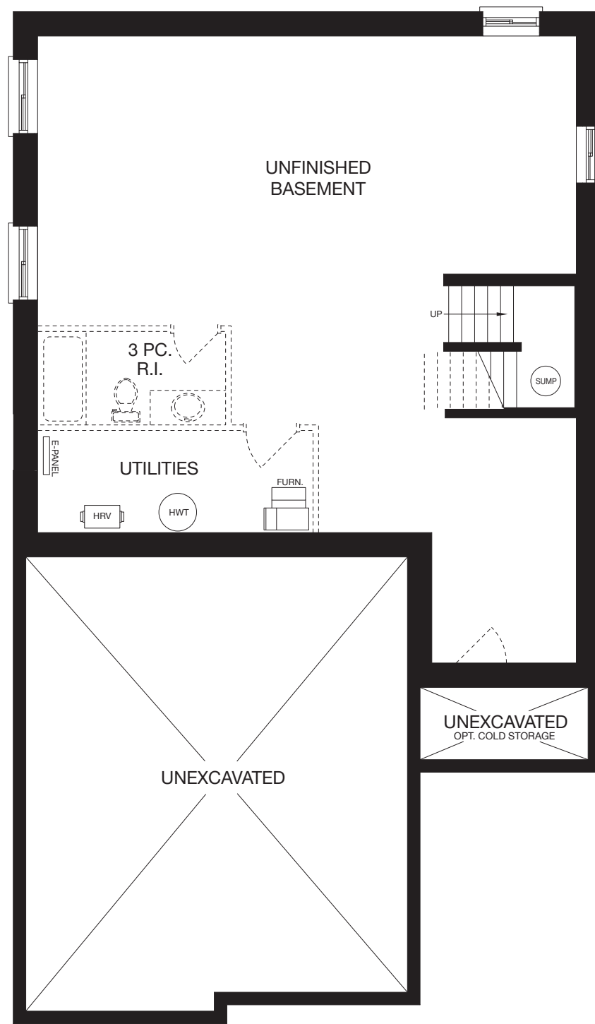
Basement
