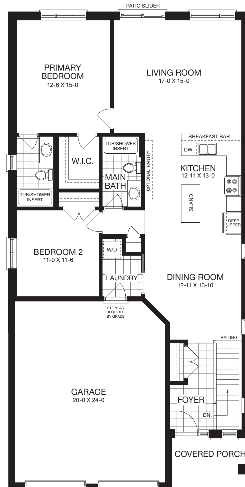
MAIN FLOOR
